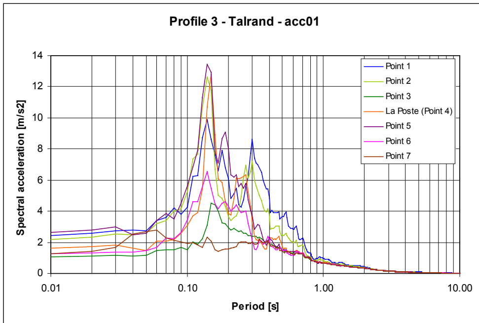
Figure 9. Strong basin edge effect observed at different points along the edge of the valley
