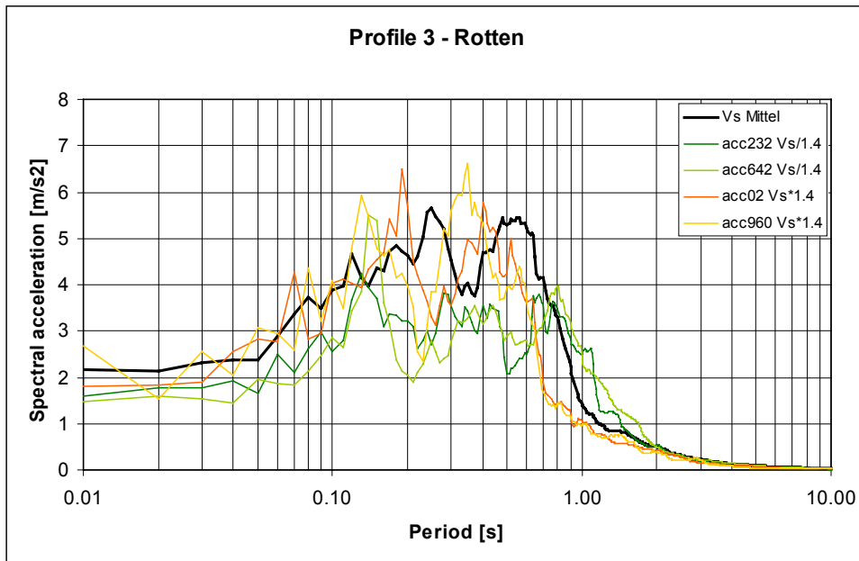
Figure 7. Amplification functions obtained with the mean (black curve) and varied velocity profiles
