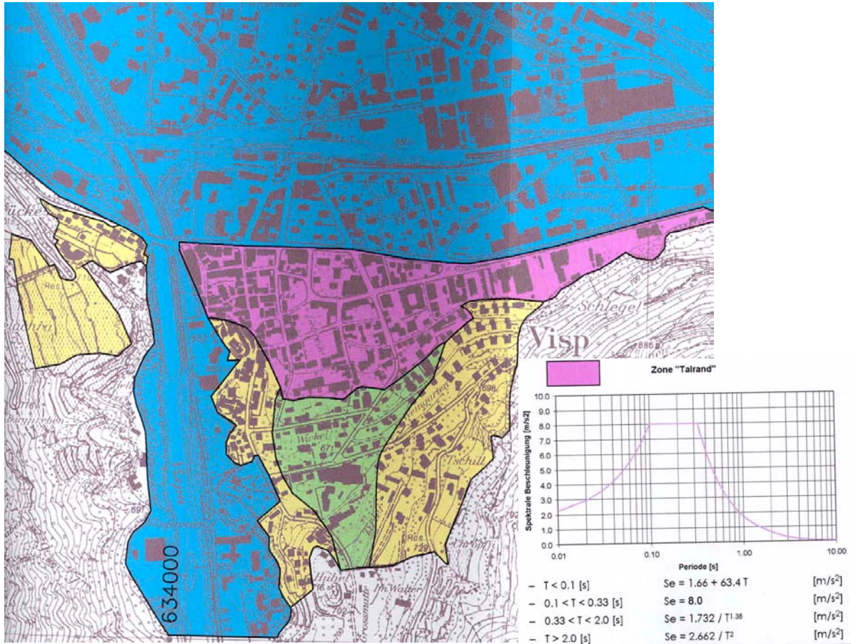
Figure 12. Extract of the seismic microzonation map of Visp
