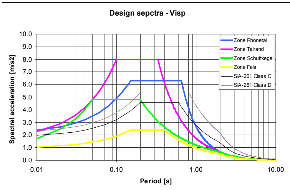
Figure 13. Proposed elastic design spectra in each zone, compared to the code spectra, that would be used without accounting for the specific 2D site effects (in grey)
